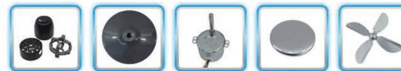
水滴状 拉伸圆形机壳配前后花篮 round wrought iron crust motor housing 新款圆形底座 latest-design round plastic base 同步电机 synchronous motor b-型新款前网装饰环 b-type latest-design decorative panel for front grill 大角度4铝叶 big-angle 4 aluminum blade
